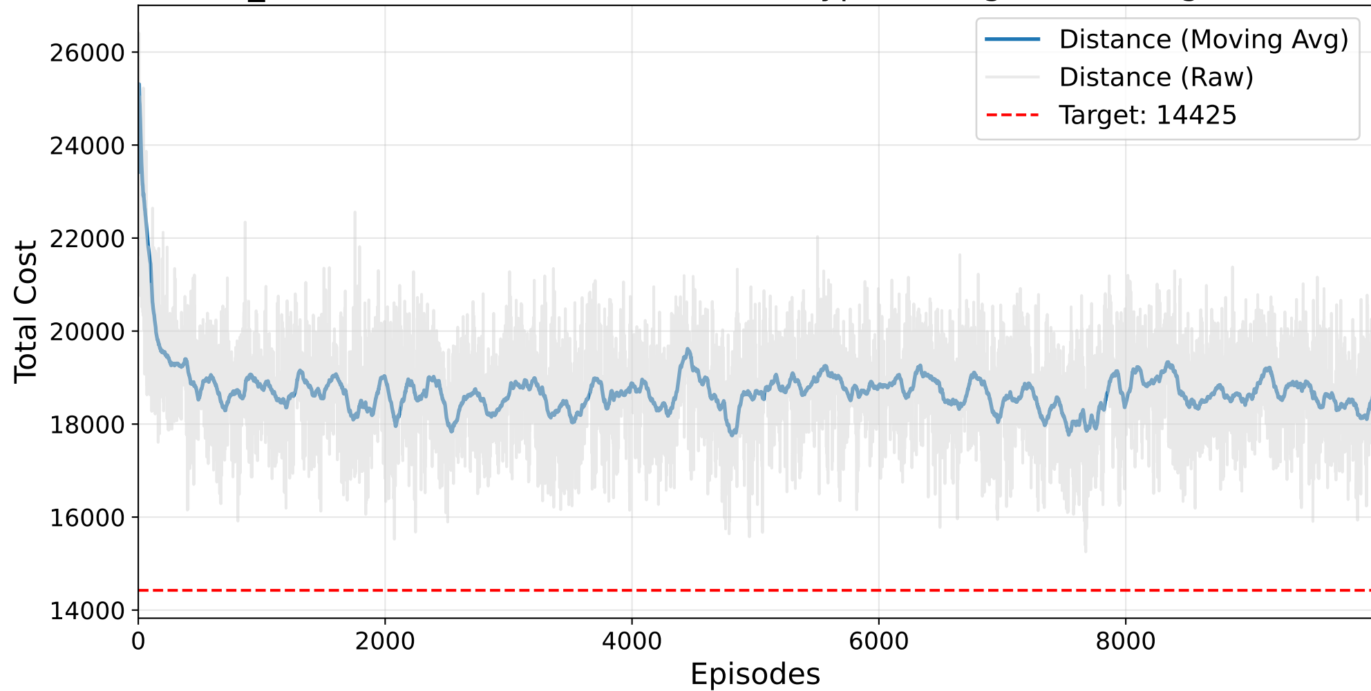
Final NO_BAYESIAN Masked AutoRL-SOP (HyperTuningSK) Training - ft53.4.sop
